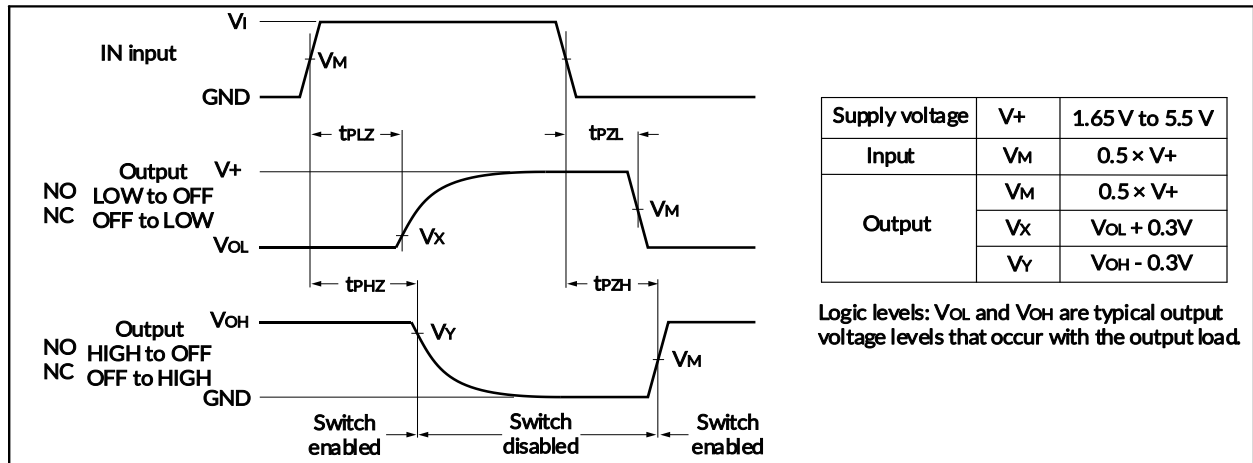
Figure 14. Turn-On ( t_{ON} ) and Turn-Off Time ( t_{OFF} )
