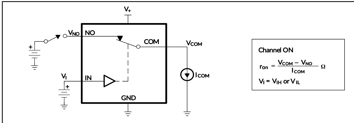
Figure 8. ON-State Resistance ( R_{on} )
