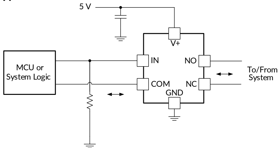
Figure 21. System Schematic for RES3157
