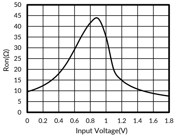
Figure 3. Typical Ron as a Function of Input Voltage ( V_+ = 1.8\text{ V} )
