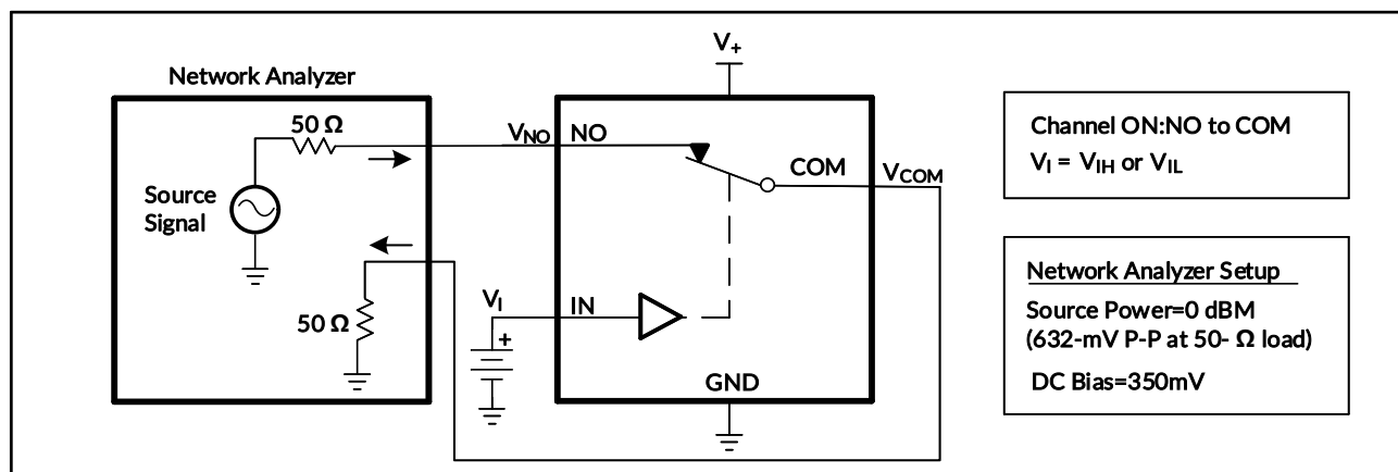
Figure 10. Bandwidth (BW)
