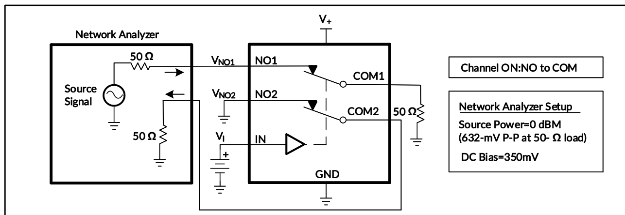
Figure 12. Crosstalk ( X_{TALK} )
