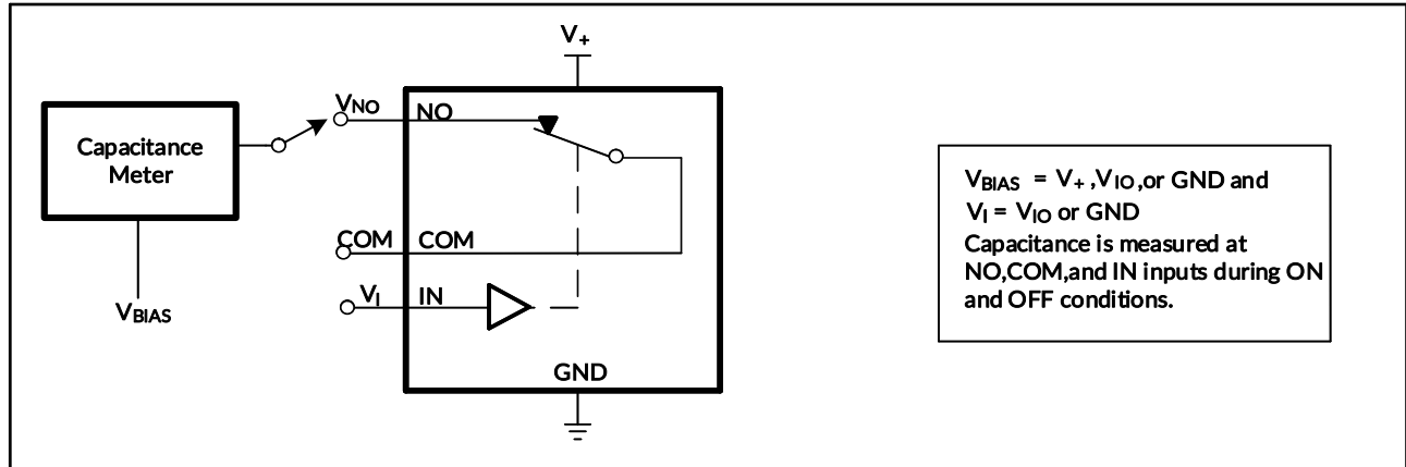
Figure 7. Capacitance ( C_I , C_{COM(ON)} , C_{COM(OFF)} , C_{NO(ON)} , C_{NO(OFF)} )
